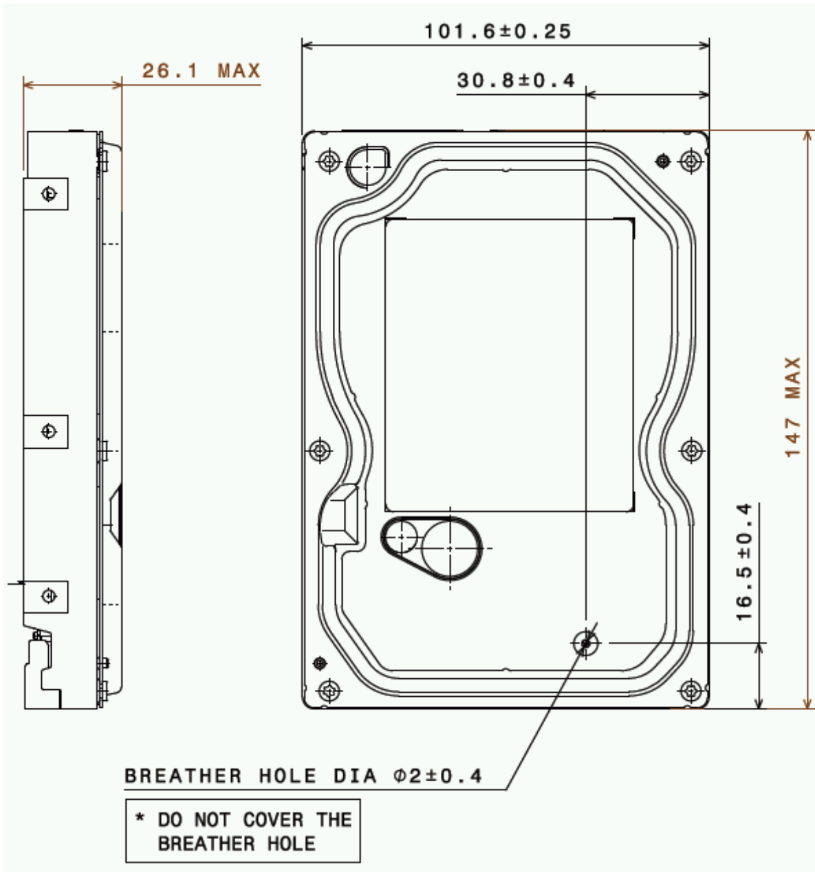
Figure 6 1D model Top and side views with breather hole location and mechanical dimensions
