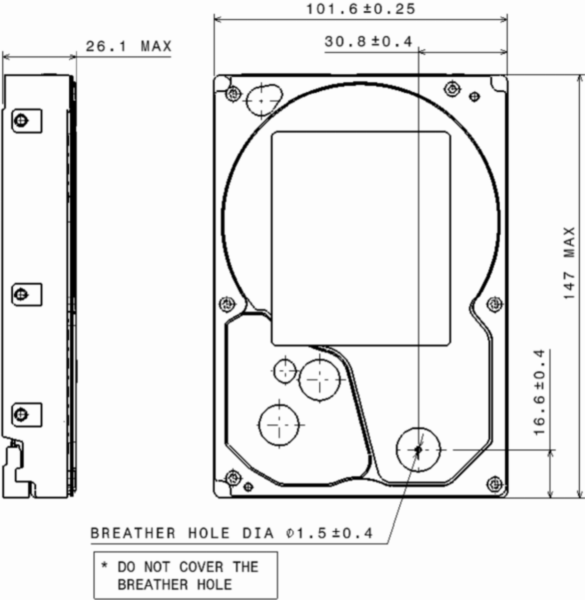
Figure 5 Top and side views with breather hole location and mechanical dimensions
